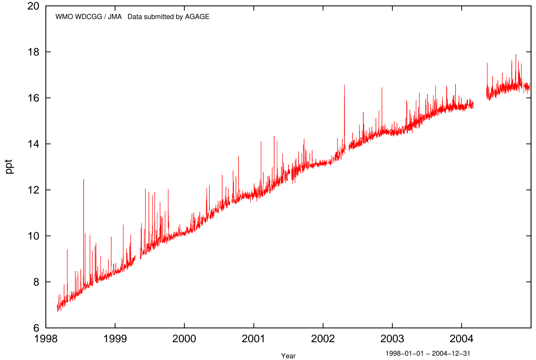
Cape Grim 40.680S, 144.680E 94m HCFCs (continuous) hcfc141b (ms) event
