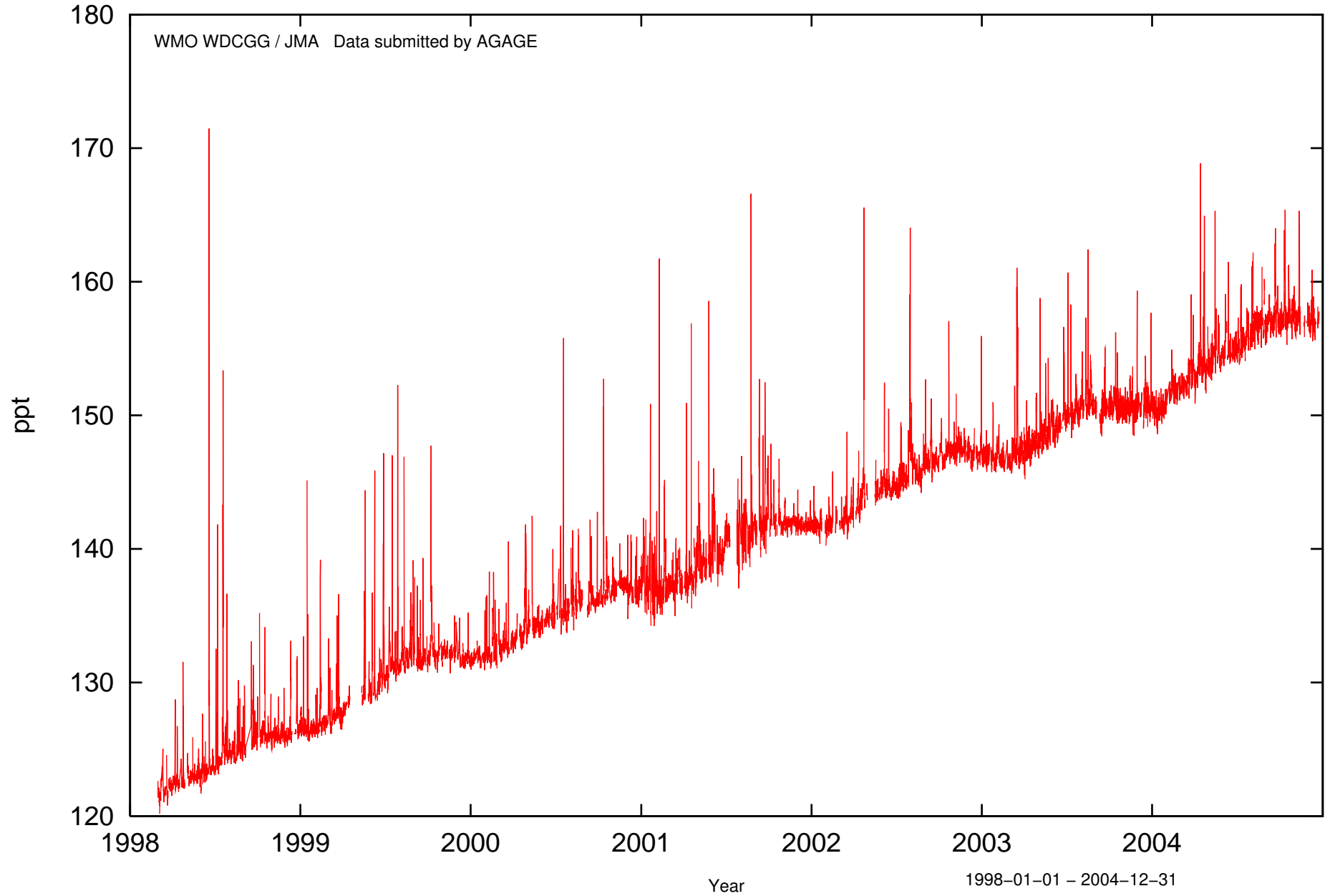
Cape Grim 40.680S, 144.680E 94m HCFCs (continuous) hfc22 (ms) event
