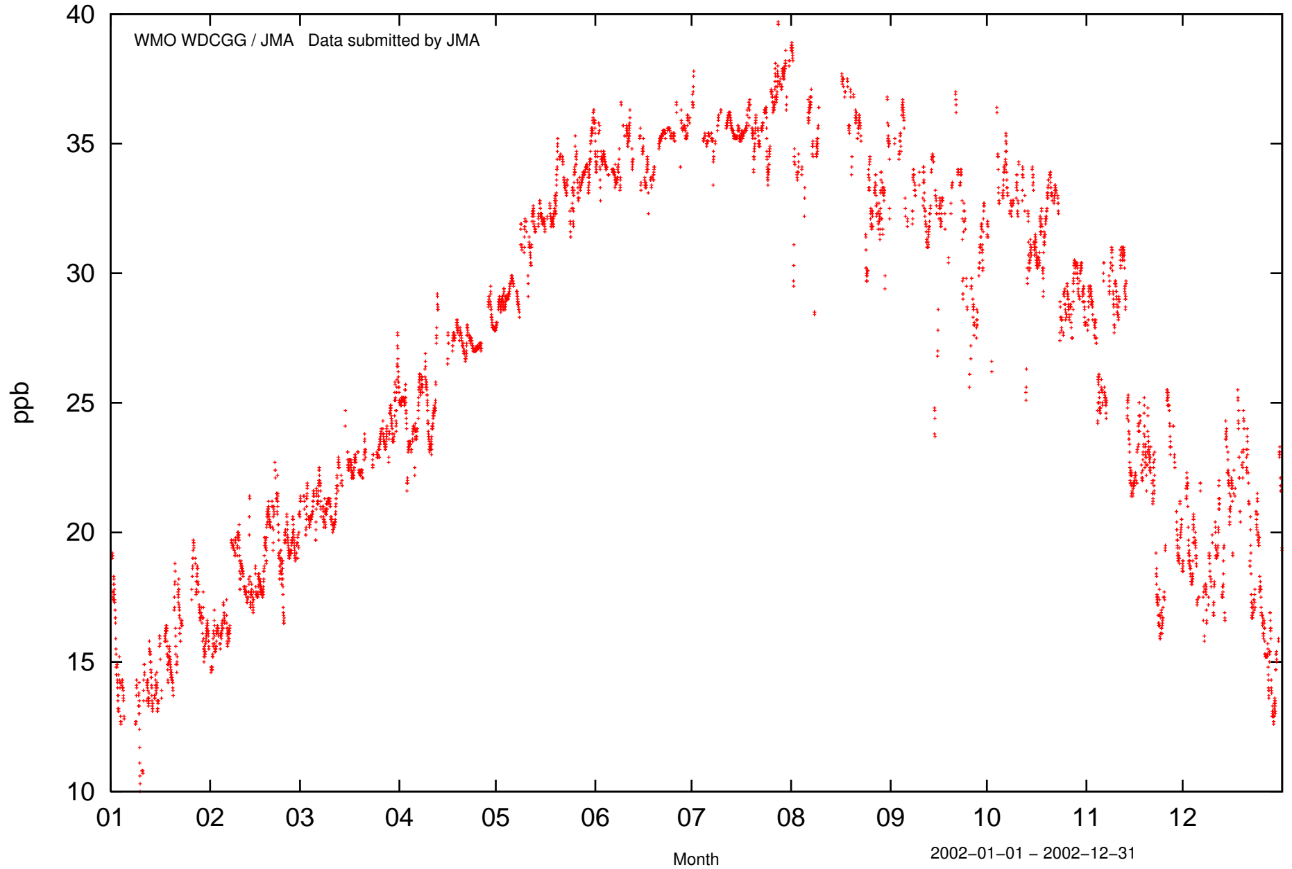
Syowa Station 69.000S, 39.580E 16m O3 (continuous) hourly
