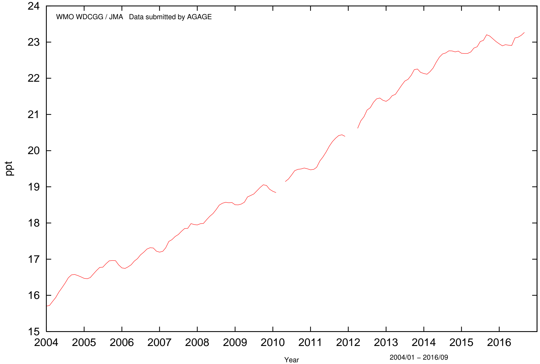
Cape Grim 40.680S, 144.680E 94m HCFCs (continuous) hfc141b (medusa) monthly
