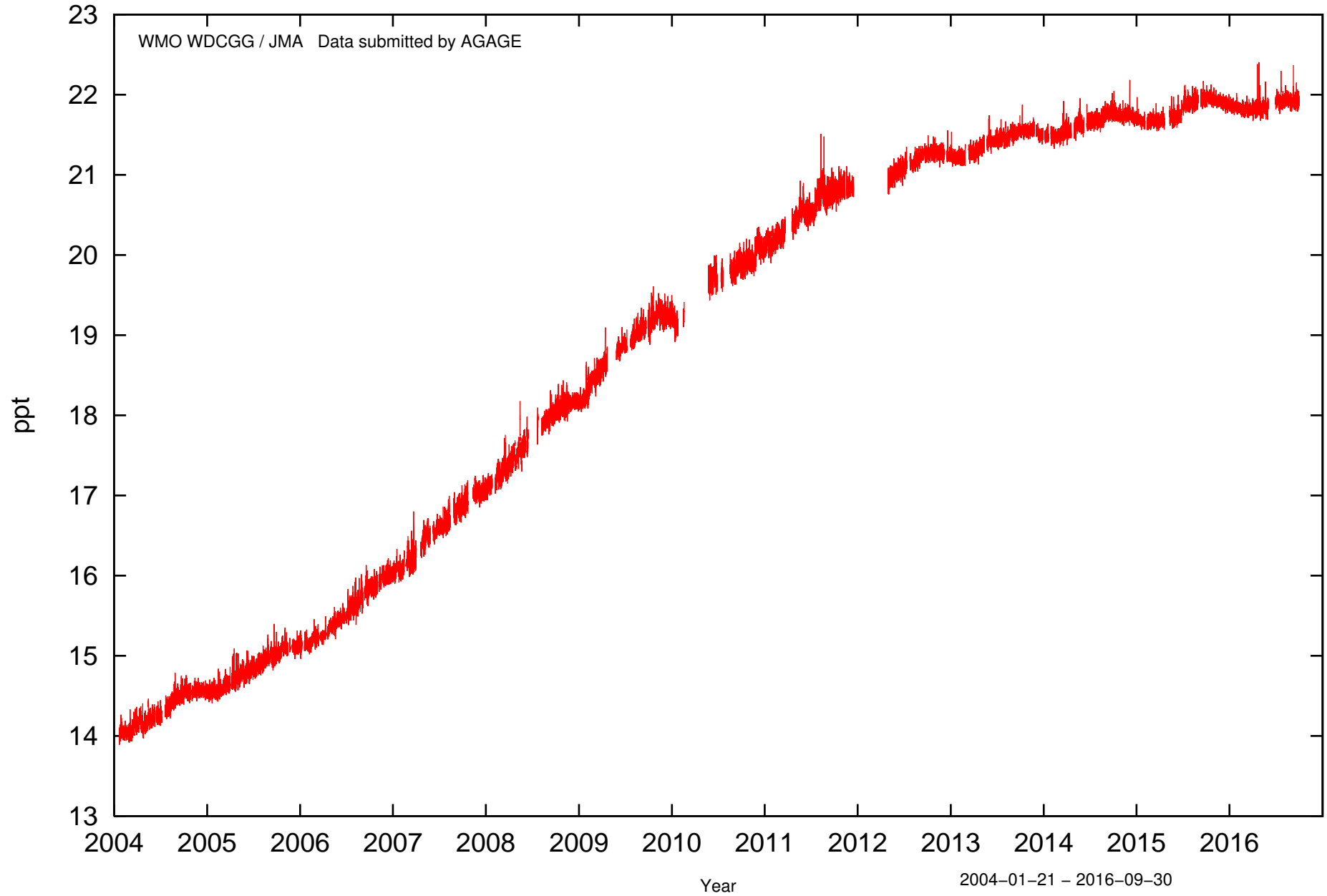
Cape Grim 40.680S, 144.680E 94m HCFCs (continuous) hcfc142b (medusa) event
