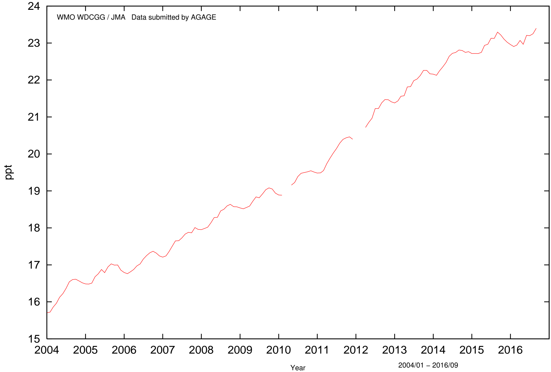
Cape Grim 40.680S, 144.680E 94m HCFCs (continuous) hfc141b (medusa_p) monthly
