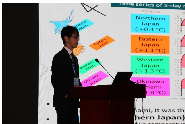
Akira Ito presenting seasonal forecast for this summer (left) and Masashi Sumitomo presenting characteristics of the last winter monsoon (right) at FOCRA II.
