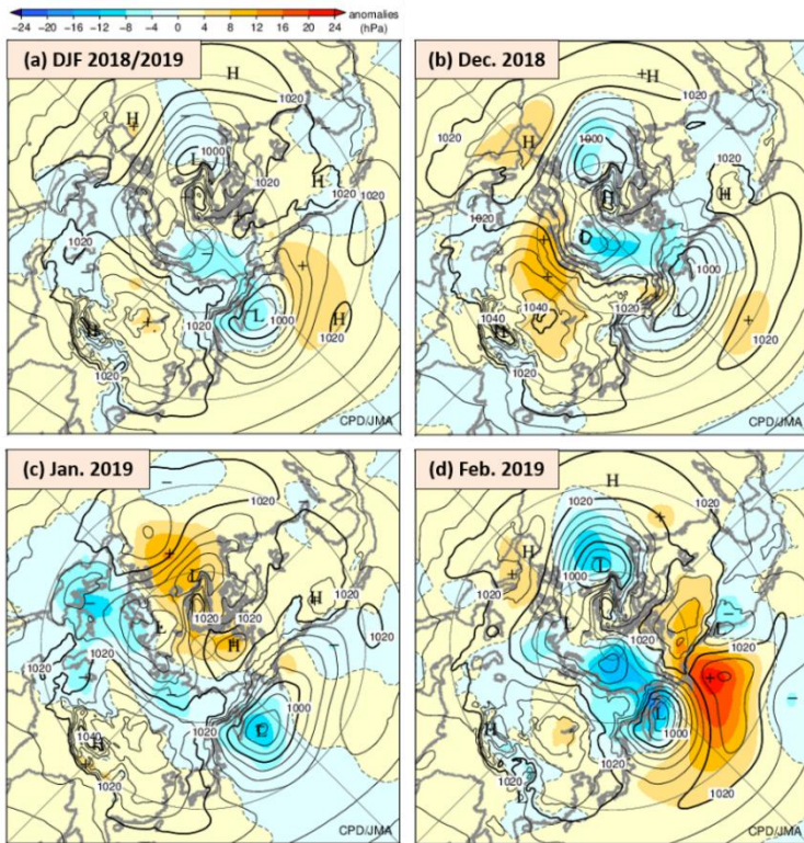
Figure 24 Sea level pressure [hPa] (a) averaged over the three months from December 2018 to February 2019, for (b) December 2018, (c) January 2019 and (d) February 2019. The contours indicate sea level pressure at intervals of 4 hPa, and the shading shows related anomalies. H and L indicate the centers of high and low pressure systems, respectively, and + (plus) and - (minus) show the peak and bottom of sea level pressure anomalies, respectively.
