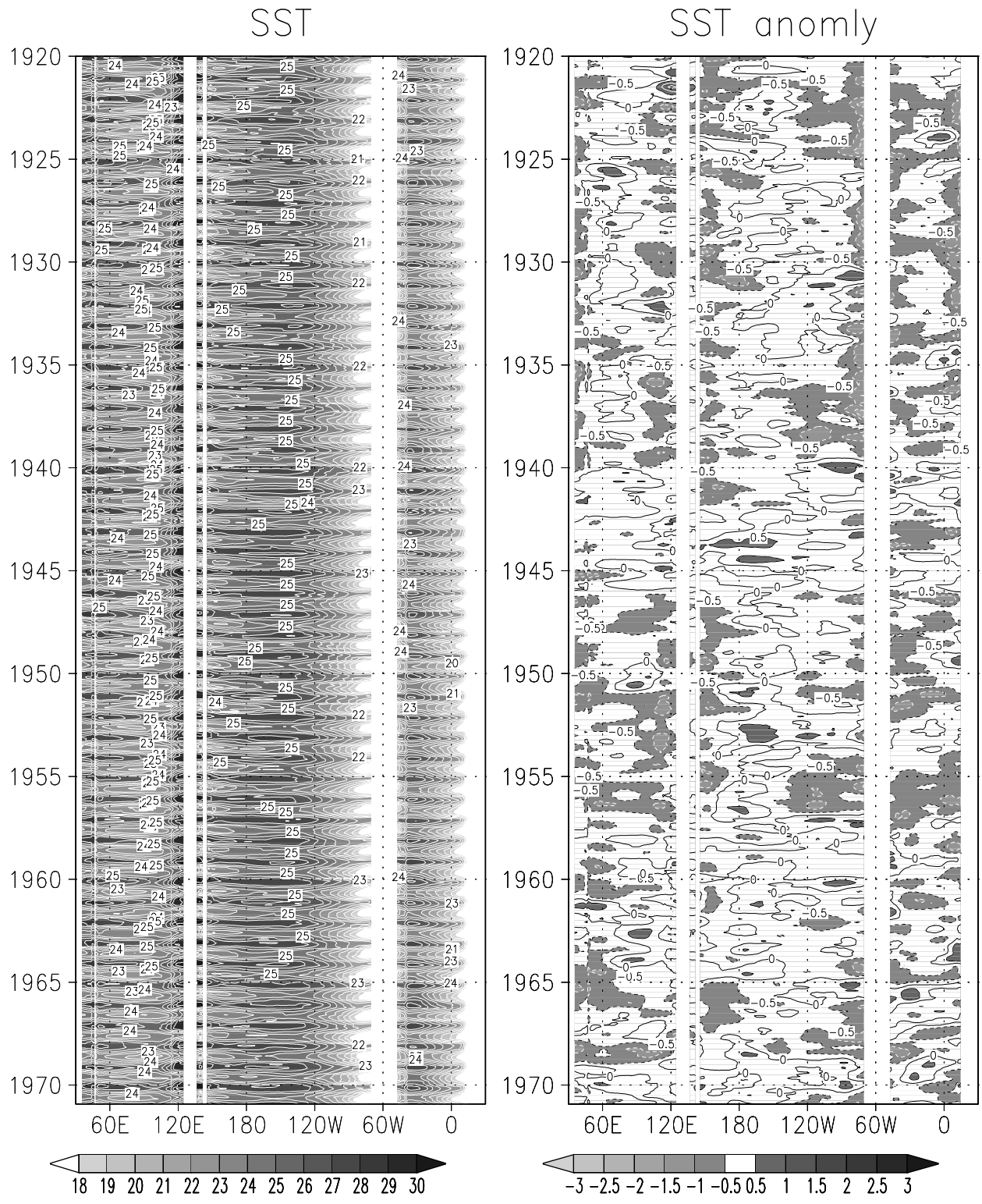
TIME-LONGITUDE SECTION OF MEAN AND ANOMALOUS SEA SURFACE TEMPERATURE FOR 15°S-25°S.
