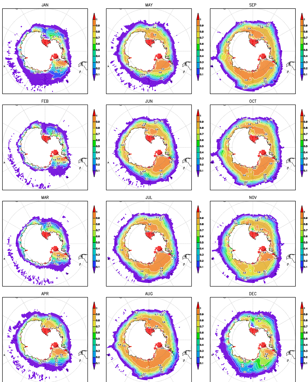
MONTHLY MEAN NORMAL OF SEA ICE CONCENTRATION (SOUTHERN HEMISPHERE) Period for normal is written in the top title. The target month is written in the title of each map. Each 1^{\circ} \times 1^{\circ} box is colored according to the value. Contour interval is 0.1.
