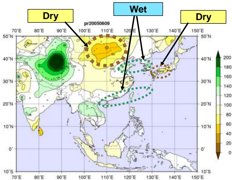
Four-month precipitation ratio (%) (Jun-Sep 2005)
