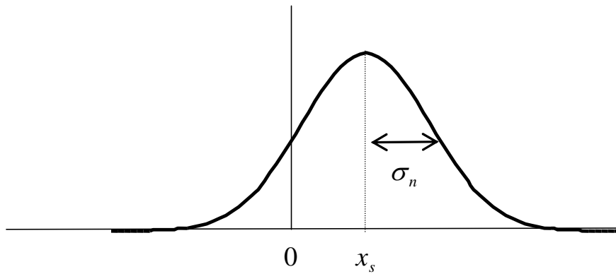
Figure 4 Schematic diagram of forecast probability density function (PDF)
