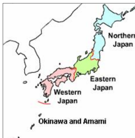
Figure 8 Outlook for winter 2011/2012 temperature probability in Japan
