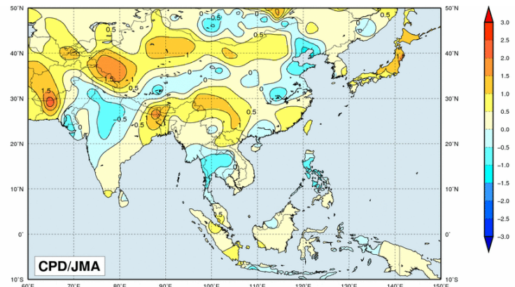
Figure 15 Four-month mean temperature anomalies (°C) from June to September 2011
