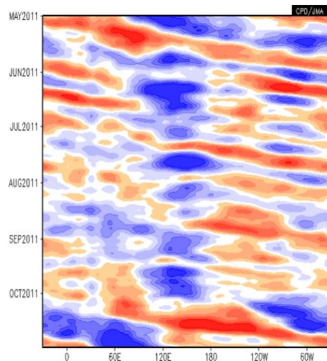
Figure 12 Time-longitude cross section of five-day running mean 200-hPa velocity potential anomaly from May to October 2011 (5°S – 5°N mean)
