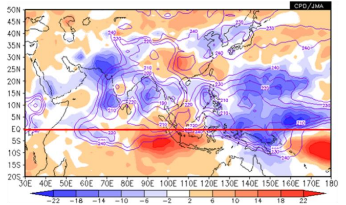
Figure 10 Four-month mean outgoing longwave radiation (OLR) and its anomaly for June – September 2011
