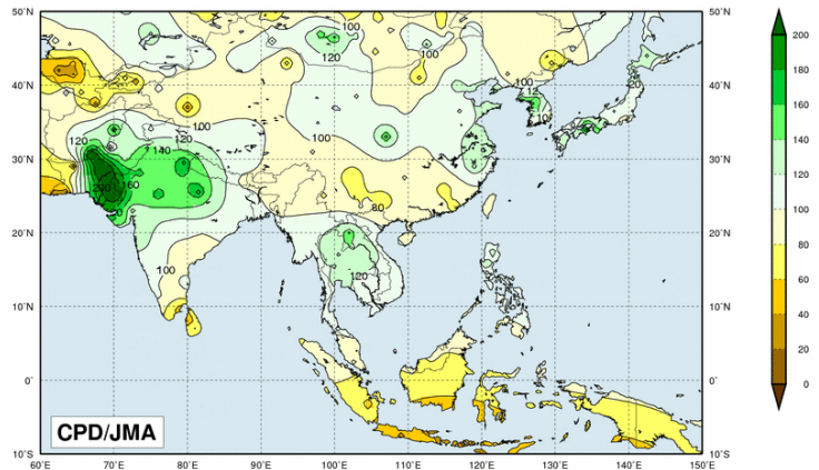
Figure 14 Four-month precipitation ratios (%) from June to September 2011
